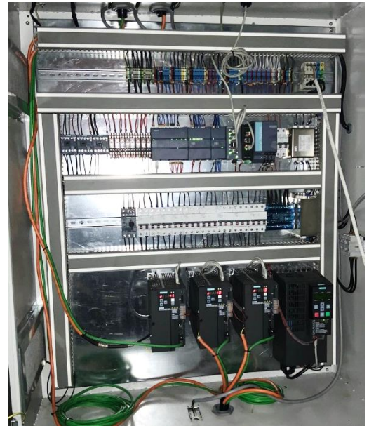
Electrical Cabinet Siemens
